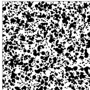
Figure 6.8 – Pitting Chart for Grade 3 Pitting Corrosion
