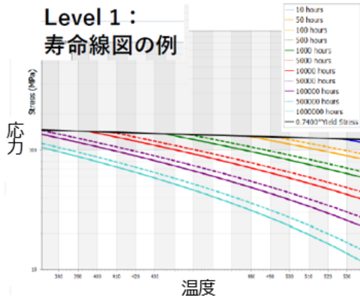
Figure 10.3M – Level 1 Screening Curve for Carbon Steel – \sigma_{allow}^{min} < 413 \text{ MPa}
