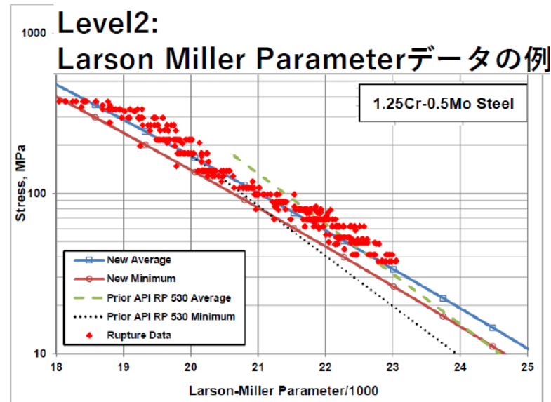
Figure 15.6-2M – The Average and Minimum Stress-Rupture Strengths as Functions of the Larson-Miller Parameter – Comparison of Existing API Std 530 Data and New Data in Metric Units Based on the Average Larson-Miller Constant: 1.25Cr-0.5Mo
