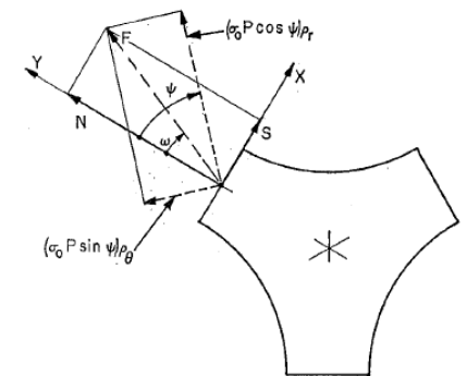
Fig. 1(b) Loads acting in minimum ligament section
