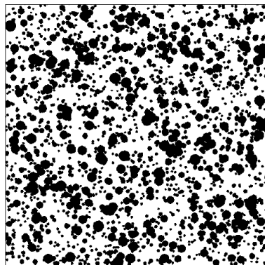
Figure 6.7 – Pitting Chart for Grade 2 Pitting Corrosion
